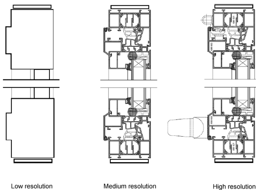
Figure 3 Grade of detail for a tilt-turn window
